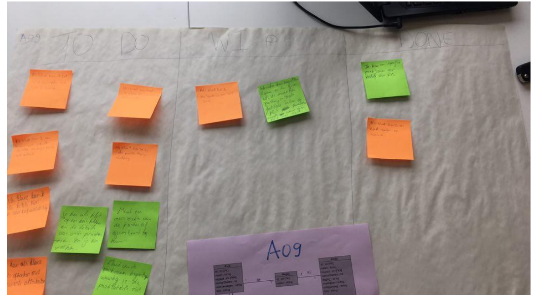
Scrum-board
